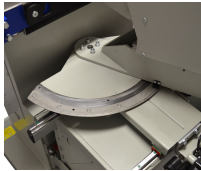
Bohraggreat schwenkbar - 65° - 0 - 65°
